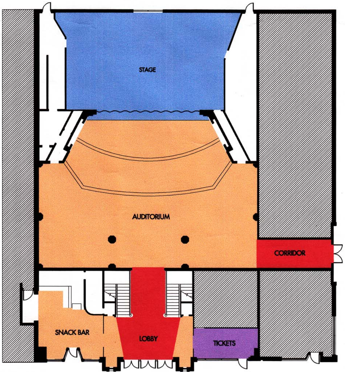
1 FIRST FLOOR PLAN
